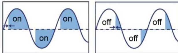
Figure 4: Leading-edge dimming
