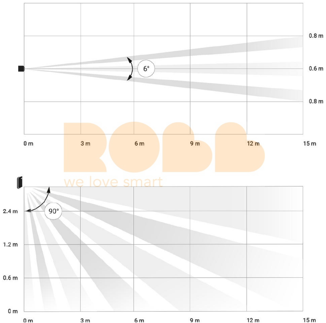
Horizontal and vertical detector's angles of view
