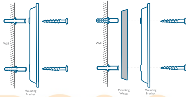
Without 15° Mounting Wedge
