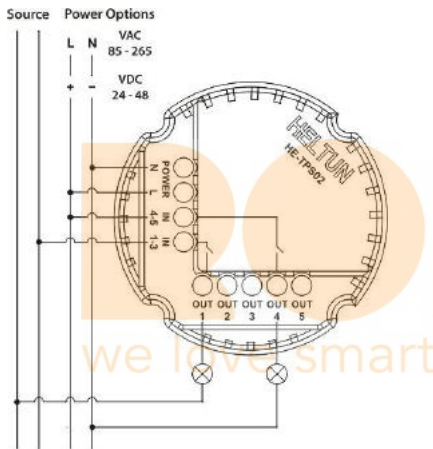
Connection Diagram 3
