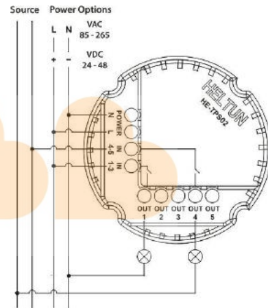
Connection Diagram 4
