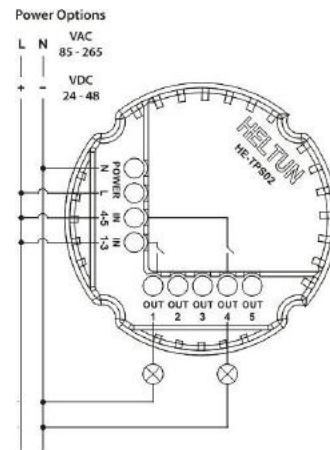
Connection Diagram 2
