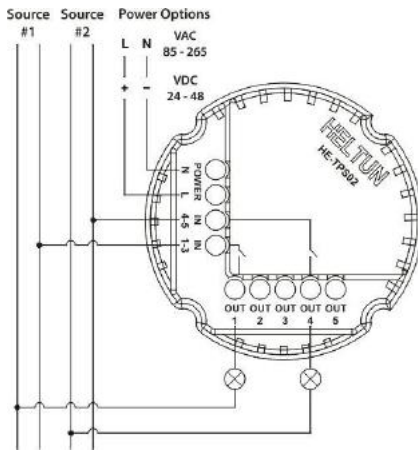
Connection Diagram 1
